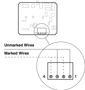
TD1 Probe Connections
