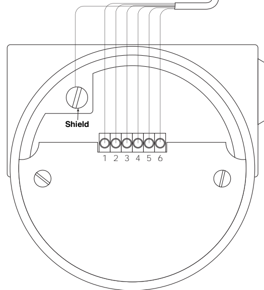
Remote TD2 Wiring
